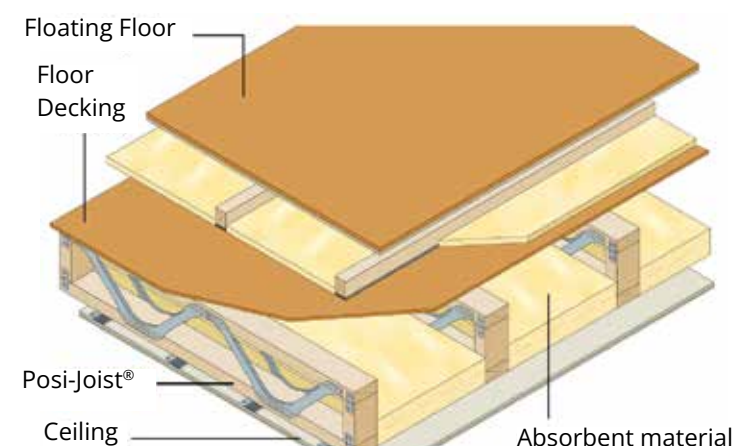
Separating floor construction (Robust Detail E-FT-3)
