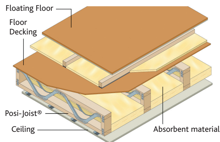
Separating floor construction (Robust Detail E-FT-3)
